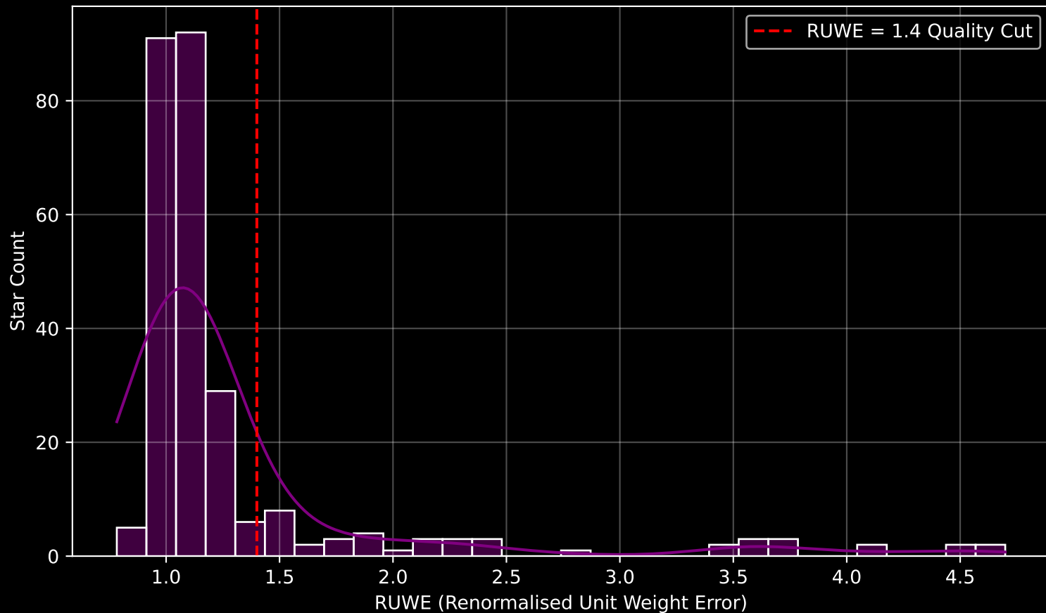
GALAH DR4 Field [9336] RUWE Distribution (n= 265)
