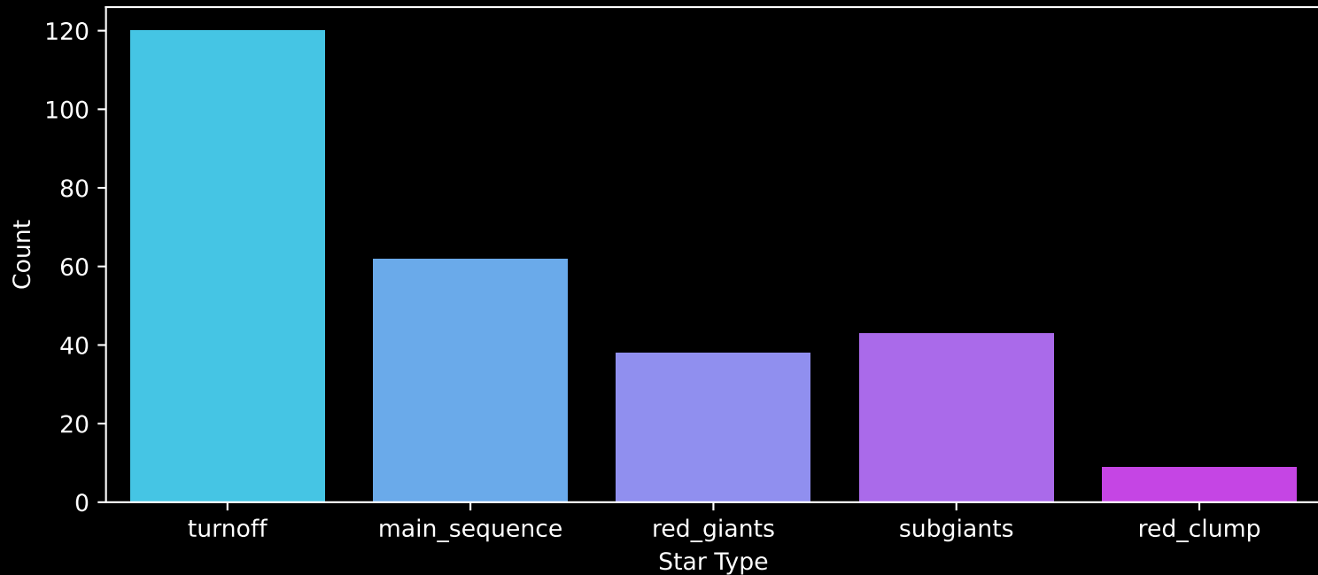
GALAH DR4 Field: [9336] Count plot of Star Type
