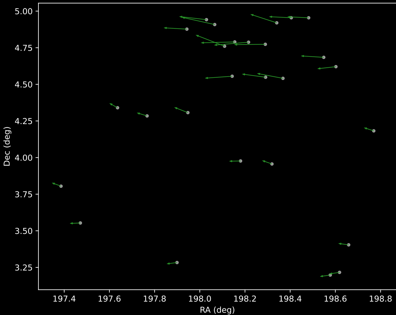
GALAH DR4 Cluster 4 Proper Motion Vectors (n=27)
